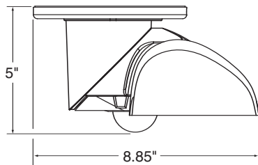
Soffit-Mounted Configuration
